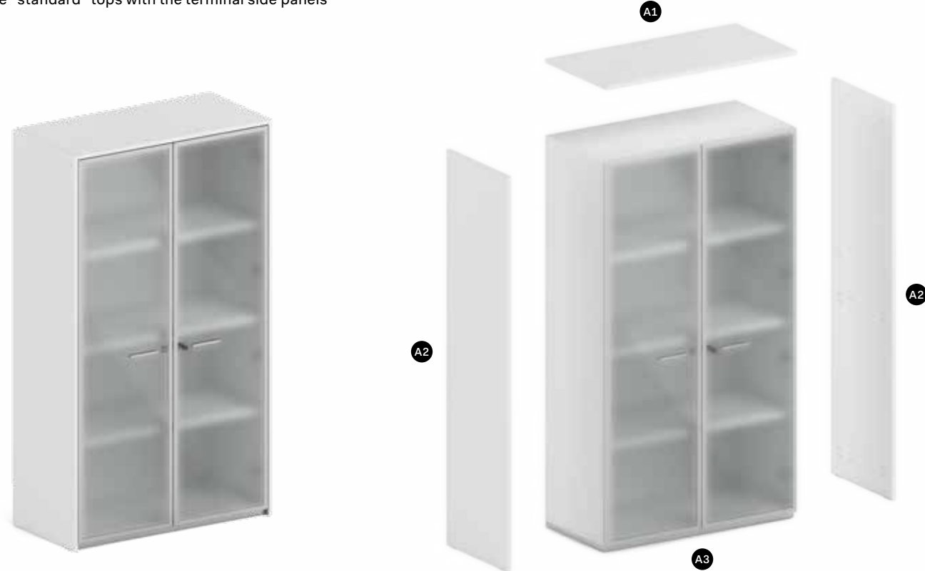
A1 Top "standard": sp. 1.8 cm / "Standard" top: 3/4" thick
